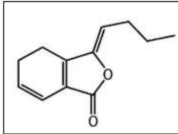
Figure 23 : Ligustilide
