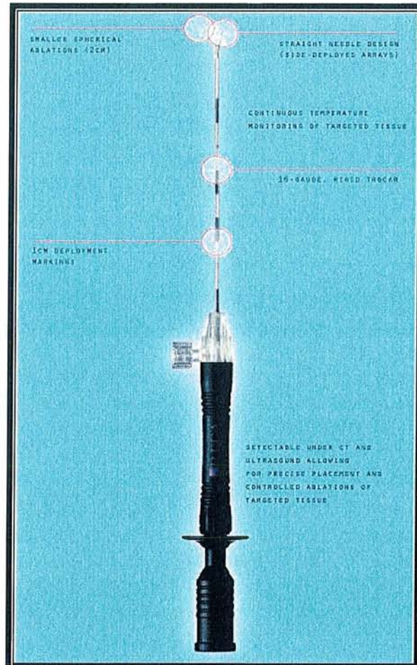
Figure 5 : aiguille STARBURST®
