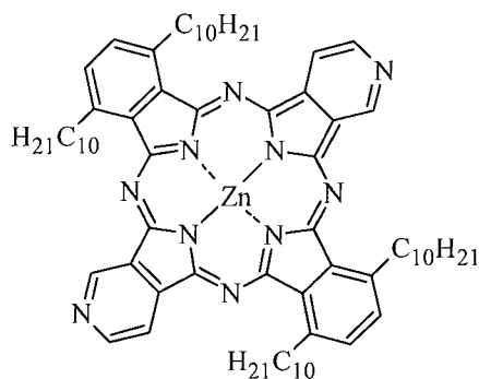
Figure 28 : bis(1,4-didécylbenzo)-bis(3,4-pyrido)porphyrazine de zinc
