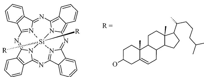
Figure 40 : dicholestéryl métallophtalocyanine de silicium \lambda_{\text{max}} = 670 \text{ nm} , \epsilon = 276690 \text{ M}^{-1} \cdot \text{cm}^{-1} (THF) [69]
