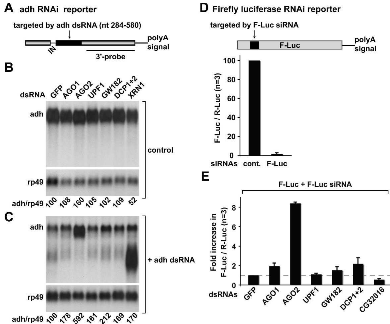
FIGURE 2. siRNA-mediated gene silencing occurs independently of NMD or the miRNA pathway. (A) Schematic representation of the adh reporter as described by Orban and Izauralde (2005). (Gray boxes) exons; (black box) sequences complementary to the dsRNAs; (IN) intron. The region of the transcript detected by the 3' probe used in panels B and C is indicated. (B,C) S2 cells constitutively expressing adh mRNA were treated with the dsRNAs indicated above the lanes. In panel C, cells also were treated with adh dsRNA. The levels of the reporters were quantitated and normalized to those of rp49 mRNA. These values were set to 100 in cells treated with GFP dsRNA. (D) Schematic representation of the firefly luciferase RNAi reporter. The region complementary to F-Luc siRNA is shown in black. S2 cells were transfected with plasmids expressing firefly and Renilla luciferase (F-Luc and R-Luc, respectively). siRNAs targeting firefly luciferase (F-Luc siRNA) or a control siRNA (cont.) were cotransfected. Four days post-transfection, firefly and Renilla luciferase activities were measured in three independent experiments ( n = 3 ). Firefly luciferase activity was normalized to that of Renilla and set to 100 in cells treated with control siRNA. Mean values \pm standard deviations are shown. (E) S2 cells were treated with the indicated dsRNAs. Six days after the first knockdown, cells were transfected with plasmids expressing firefly and Renilla luciferase, and either F-Luc or control siRNAs. Firefly and Renilla luciferase activities were measured 4 d post-transfection. For each knockdown, firefly luciferase activity was normalized to that of the Renilla and set to 100 in cells transfected with control siRNA (not shown). The normalized luciferase activity in cells transfected with F-Luc siRNA and treated with GFP dsRNA was then set to 1. Mean values \pm standard deviations are shown.
