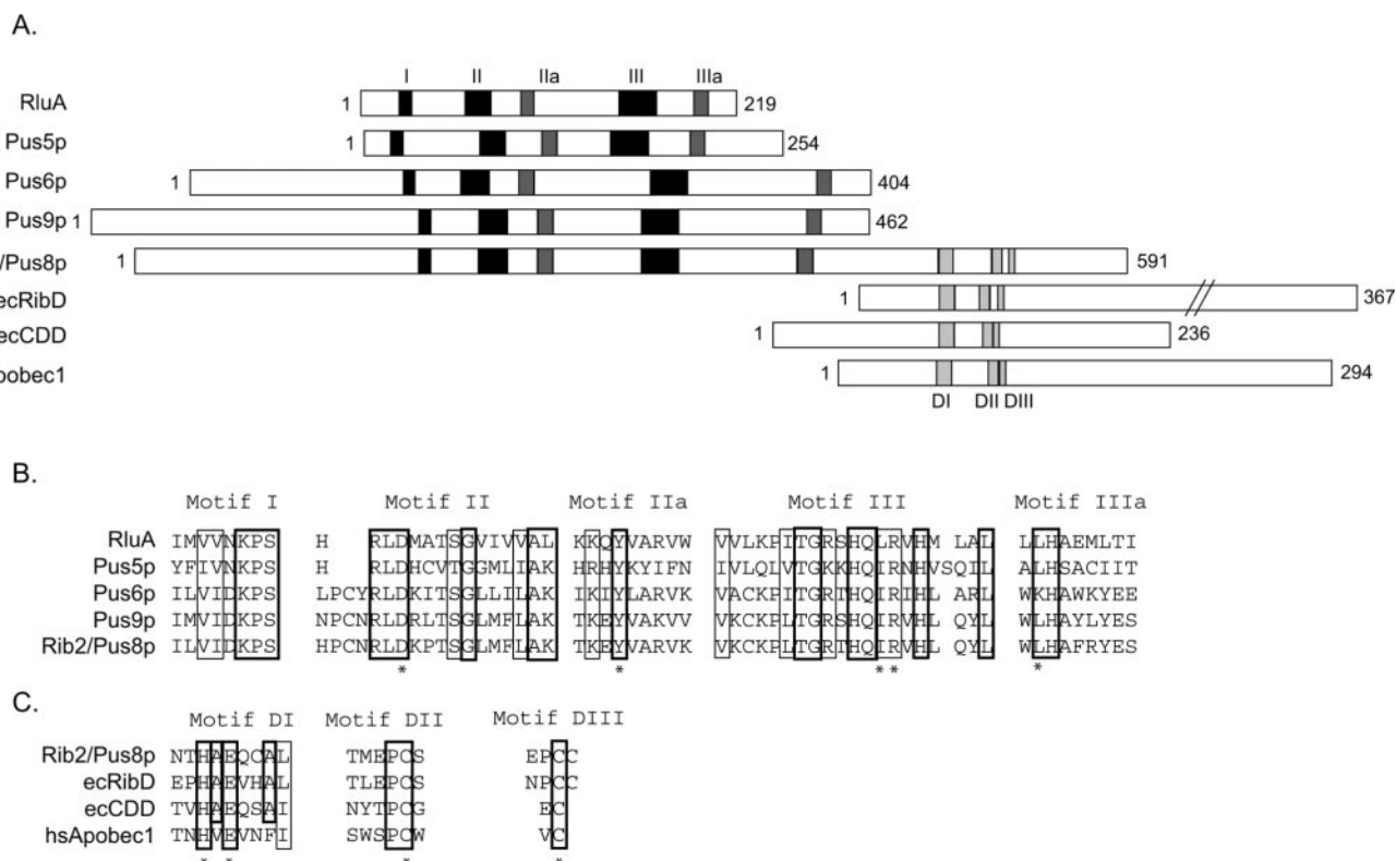
FIG. 2. The Rib2/Pus8p protein sequence contains both an RNA: \Psi -synthase and a deaminase domain. A , schematic representation of the sequence alignment of the yeast Pus5p, Pus6p, Pus9p, and Rib2/Pus8p RNA: \Psi -synthases, together with the E. coli RluA, RibD ( ecRibD ) and cytosine deaminase ( ecCDD ) enzymes and the human Apobec I deaminase ( hsApobec1 ). The five conserved motifs I, II, Ila, III, and IIIa of RNA: \Psi -synthases are represented by black and dark gray rectangles (43). The three specific motifs (DI, DII, and DIII) of deaminases are represented by gray rectangles (44). B , the amino acid sequence alignment of motifs I, II, Ila, III, and IIIa of the RluA, Pus5p, Pus6p, Pus9p, and Rib2/Pus8p enzymes. Identical and semi-conserved residues are boxed. The thickness of the line corresponds to the level of conservation. The conserved residues (D, Y, I, R, and L) in the various RNA: \Psi -synthases active sites are indicated by asterisks. C , the amino acid sequence alignment of motifs DI, DII, and DIII of the Rib2/Pus8p, EcRibD, EcCDD, and hsApobec1 deaminases. As in B , identical and semi-conserved residues are boxed, and the thickness of the line corresponds to the level of conservation. The conserved residues (H, E, C, and C) in the deaminases active site are indicated by asterisks.
