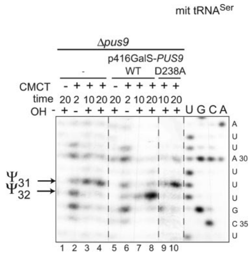
FIG. 6. The aspartic acid residue Asp-238 in the active site of Pus9p is essential for RNA:Ψ-synthase activity. The yeast S. cerevisiae \Delta pus9 strain was transformed with p416GalS plasmids, bearing the WT (Asp-238) or mutated (D238A) PUS9 ORF. Total RNA was extracted from the two transformed strains, and the mitochondrial tRNA Ser was analyzed by the CMCT/RT approach (shown in lanes 7–10). The reverse transcription stops, corresponding to residues Ψ31 and Ψ32 are indicated.
