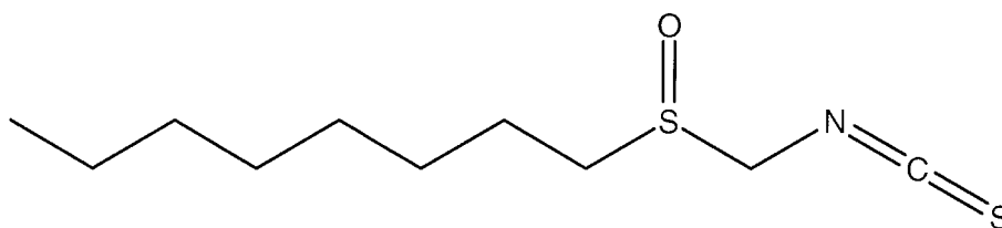
8 isothiocyanatomethylsulfinyloctane ITC8MSO
