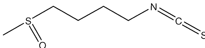
[(-)-1-isothiocyanato-(4R)(methylsulfonyl)butane] ERYSOLIN
