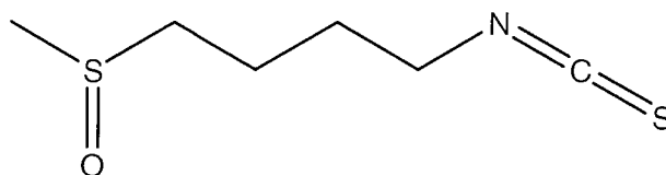
[(-)-1-isothiocyanato-(4R)-(methylsulfinyl)butane] SULFORAPHANE
