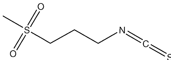
[(-)-1-isothiocyanato-(3)(methylsulfonyl)propane] CHEIROLIN
