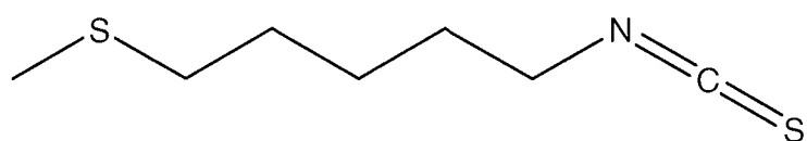
[-]-1-isothiocyanato-(5)(methylthio)pentane] BERTEROINE
