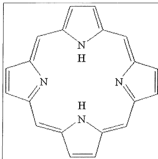
Figure 3 : Porphine
