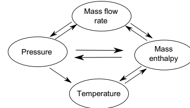
Figure 2: Networks coupling
