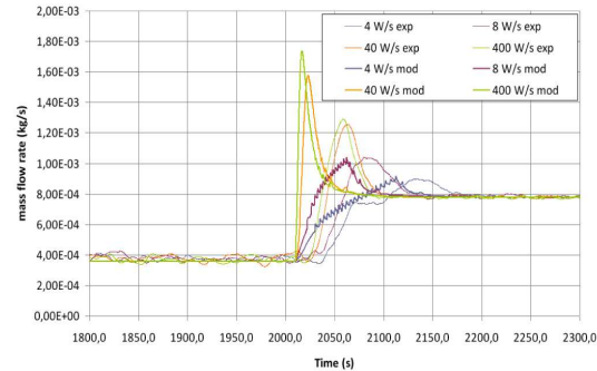
Figure 5: Outlet condenser mass flow rate responses to heat flux increases [1]
