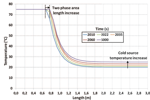
Figure 13: Iso-times temperatures in condenser during an inlet cold source temperature increase ( 0.5^{\circ}\text{C}\cdot\text{s}^{-1} )
