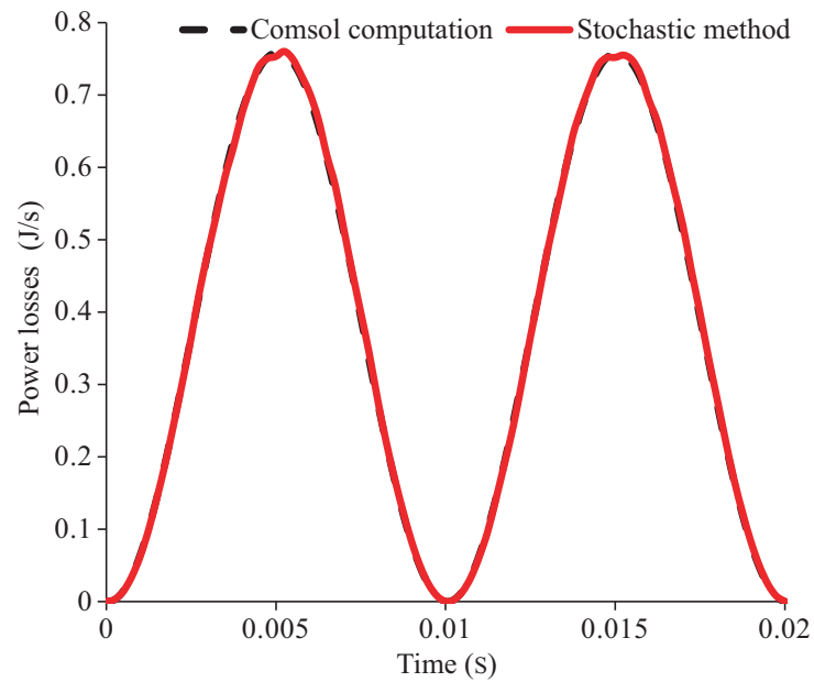
Figure 3. Calculated losses in the cooper piece versus time.
