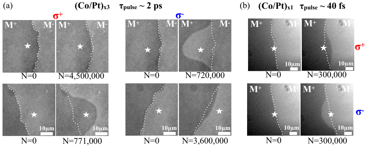
FIG. 1. Magneto-optical images of domain wall motion in [\text{Co}(0.4 \text{ nm})/\text{Pt}(0.7 \text{ nm})]_{x3} and [\text{Co}(0.6 \text{ nm})/\text{Pt}(0.7 \text{ nm})]_{x1} induced, respectively, by (a) 2-ps and (b) 40-fs laser pulses with left-circular ( \sigma^- ) and right-circular ( \sigma^+ ) polarization with an energy per pulse of 0.04 and 12.5 \text{mJ cm}^{-2} . The white star indicates the center of the beam spot, and N is the number of laser pulses. The laser beam spot is (a) placed 10 \mu\text{m} away from the DW within a magnetization-up ( M^+ ) or -down ( M^- ) domain or (b) centered on the wall. The dotted line shows the initial position of the domain wall prior to laser exposure.
