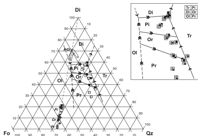
Figure 4. Liquidus boundaries in the system forsterite–diopside–anorthite–silica. Represented join is Fo 95 An 05 –Di 95 An 05 –SiO 2 95An 05 : this plane is parallel to the pseudo-ternary Fo–Di–SiO 2 diagram and contains 5% An. Squares are liquid compositions saturated with two crystalline phases (white squares) or three crystalline phases (black squares). Analyses of pyroxene crystals are shown. Single arrows indicate cotectic curves; double arrows indicate reaction curves.
