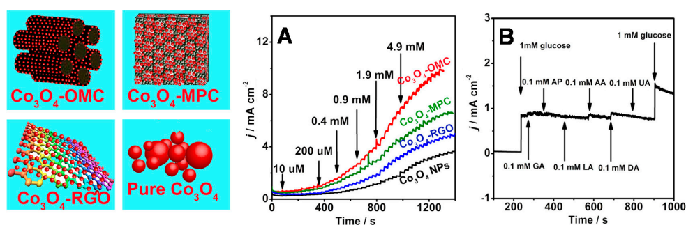
Figure 8. (A) Typical j - t curves obtained at glassy carbon electrodes (GCE) modified with Co 3 O 4 nanocrystals (GCE/Co 3 O 4 NPs), or with Co 3 O 4 nanocrystals-decorated reduced graphene oxide (GCE/Co 3 O 4 -RGO), macroporous carbon (GCE/Co 3 O 4 -MPC), and ordered mesoporous carbon (GCE/Co 3 O 4 -OMC) on the successive injection of glucose in 0.1 M NaOH solution at 0.55 V vs. Ag/AgCl, on which the concentration denoted the final glucose concentration; the corresponding modifiers are illustrated on the left. (B) The j - t curve of GCE/Co 3 O 4 -OMC with the successive addition of 1 mM glucose, 0.1 mM interference substances, and 1 mM glucose at +0.55 V vs. Ag/AgCl (reproduced from [164]).
