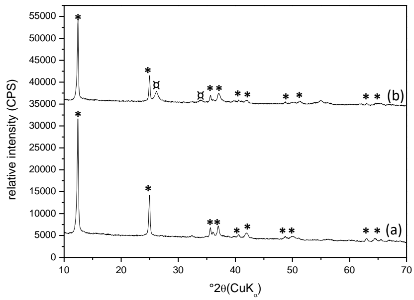
Fig. 5. XRD pattern of a) Na_2O -a and b) Na_2O -b, *Birnessite and ☒ Manganite.
