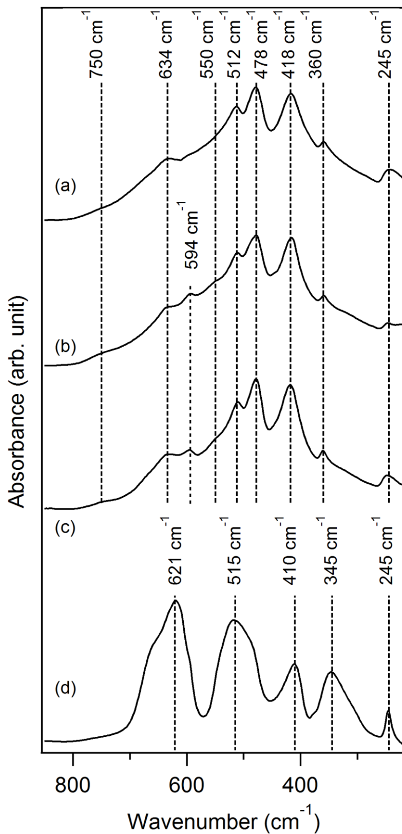
Fig. 3. IR spectra of sample (a) \text{Na}_2^R (reductant-last method), (b) \text{Na}_2^A (alkali-last method), (c) \text{Na}_2^O (oxidant-last method) and (d) hausmannite.
