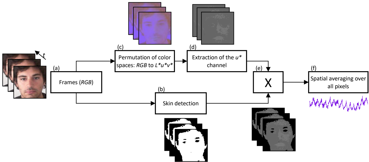
Fig. 1. Processing algorithm overview. (a) Pan, Tilt and zoom parameters are computed to zoom and track the face on the input frame. (b) Pixels that contain PPG information are isolated by a skin detection. (c) The RGB color space is converted to the CIE L^*u^*v^* color space. (d) The u^* frame is extracted and (e) merged with the skin detection mask by a combinational AND operation. (f) A spatial averaging step is performed to transform a set of frames into a single raw signal.
