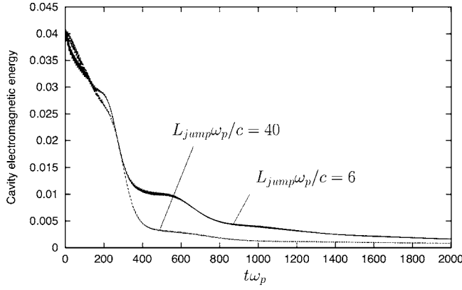
FIG. 10. The electromagnetic energy W_0 of the plasma slab cavity: the solid line corresponds to L_{\text{jump}}\omega_p/c=6 , while the dotted line is related to the case where L_{\text{jump}}\omega_p/c=40 . The depletion of the energy is, however, more rapid in the case where the slab boundaries are made sufficiently gradual.
