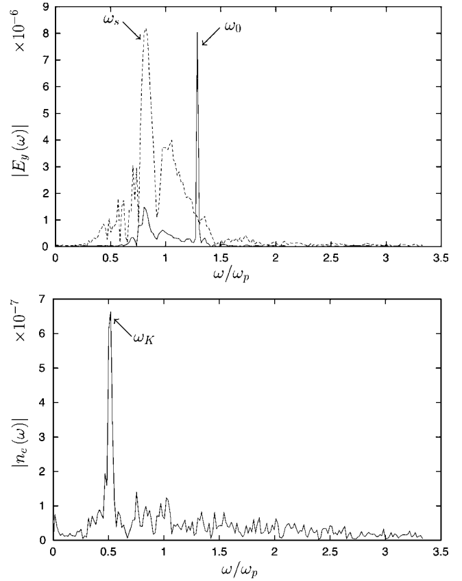
FIG. 5. The electromagnetic spectra (top panel, backward in dashed line) and electrostatic spectrum (bottom panel). The physical parameters are n_0/n_e=0.6 , a_0=0.5 .
