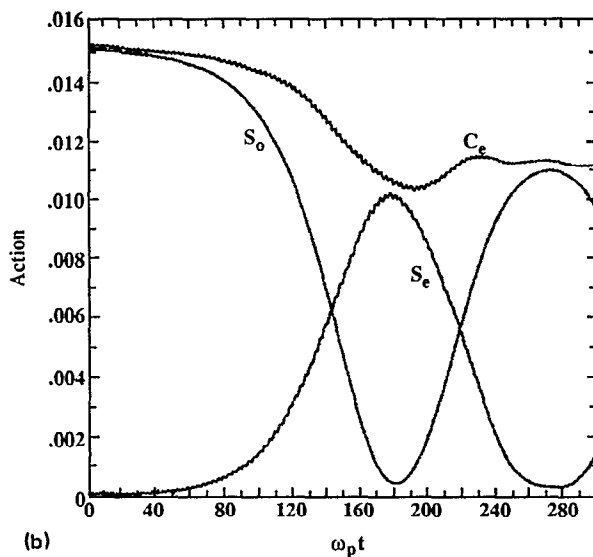
FIG. 1. From a spatially periodic initial-value Euler–Vlasov simulation of FRS: time evolution for the pump action S_0 , scattered wave action S_s , and electron plasma wave action S_e and various action sums C_s (=S_0+S_s) and C_e (=S_0+S_e) . (a) Pump S_0 , scattered FRS em wave S_s , and their action sum C_s . (b) Pump S_0 , electron plasma wave S_e , and their action sum C_e . (c) As in (b), together with C_k and C_{eT} , where C_k accounts for particle accelerated above the lower separatrix (see Fig. 5) together with the total C_{eT} (=C_e+C_k) .
