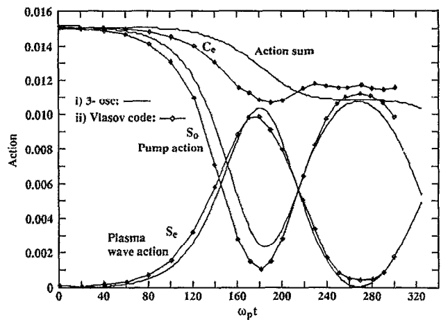
FIG. 3. Comparison of three-wave coupling (plain lines) and EVF (advanced by \omega_p t = 45 , see text) action results (lozenges). Temporal evolution of the pump and plasma actions ( S_0 and S_e ) and their action sum C_e for \gamma_e = 0.0025 \omega_p ( 1.53 \times Landau) and \Delta\omega = -0.025 \omega_p ( 1.62 \times linear calculation). Note the monotonic decrease of the action sum for the three-oscillator model contrasted with the more complex behavior due to nonlinear particle trapping effects.
