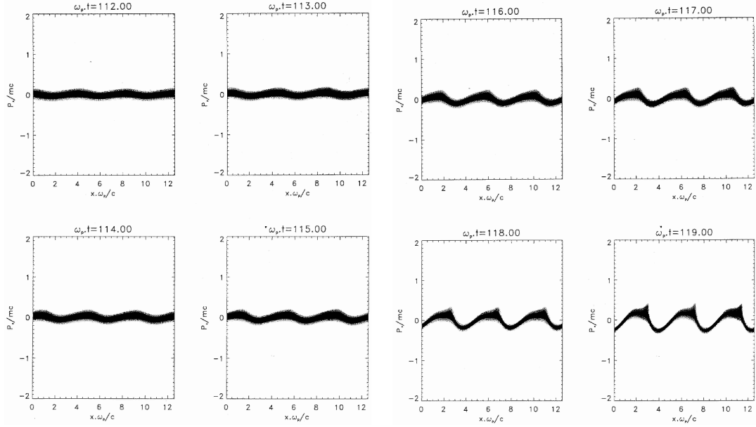
Figure 3: The x - p_x electron phase space representation afforded by the numerical Vlasov code using TSS in the case of the study of the modulational instability in the relativistic regime. The parameters of the simulation are n/n_{crit} = 0.55 , a_0 = 0.75 and k_0 c/\omega_p = 1 .
