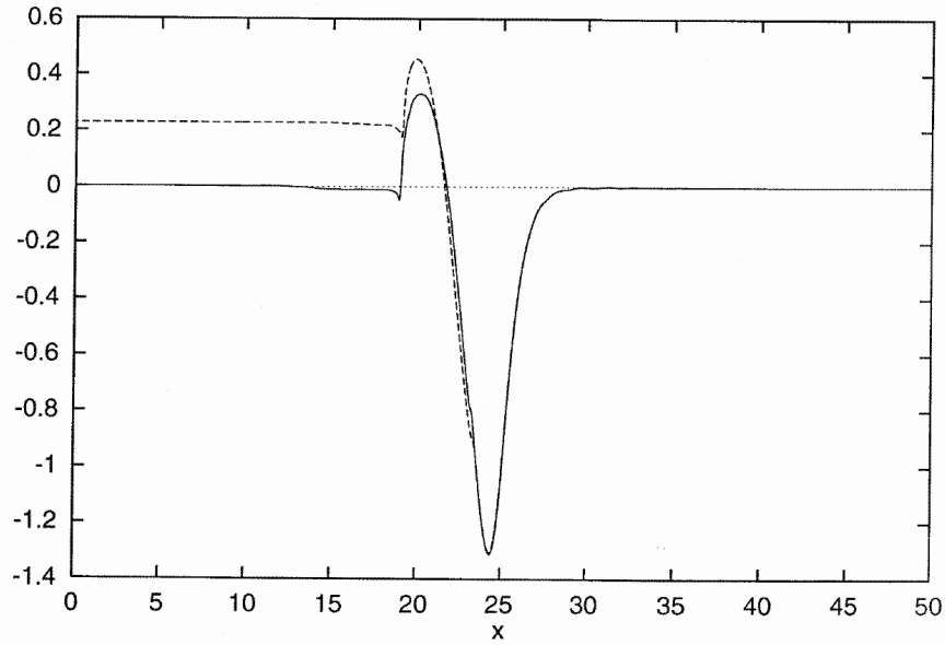
Figure 6: Behavior of the longitudinal electric field (given in m\omega_p c unit) in both simulation tests: solid line corresponds to the 2D exact advection and dotted line to TSS. A strong electric field develops at the left boundary of the plasma system (in dotted line) as the result of a bad mass conservation of the numerical algorithm based on TSS.
