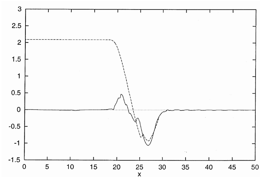
Figure 9: Display of the the longitudinal electric field versus space at time t\omega_p = 94 . A comparison between both numerical schemes of the Vlasov equation was carried out: the TSS algorithm gives rise to numerical instability in the case of integration of the relativistic Vlasov equation whereas the full 2D advection algorithm remains stable.
