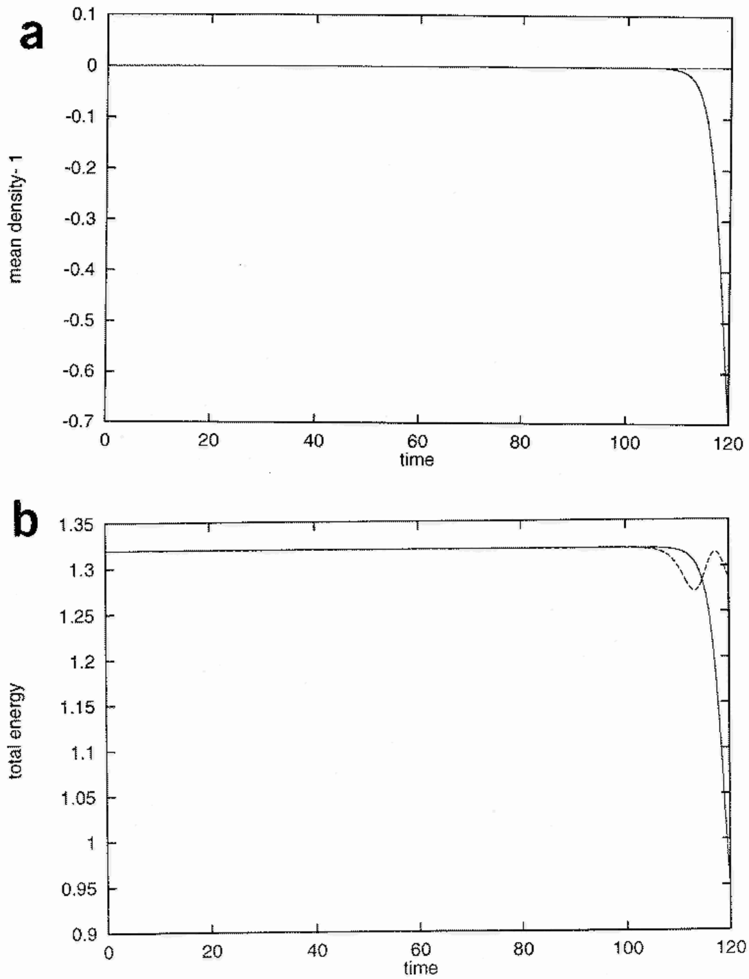
Figure 1: Numerical comparison between both Vlasov algorithms: (a) time evolution of the mean normalized density. (b) time evolution of the total energy. The full line is related to the time splitting scheme while the dotted line corresponds to the 2D full advection. Exact integration of the Vlasov equation can be achieved only by the full 2D advection algorithm.
