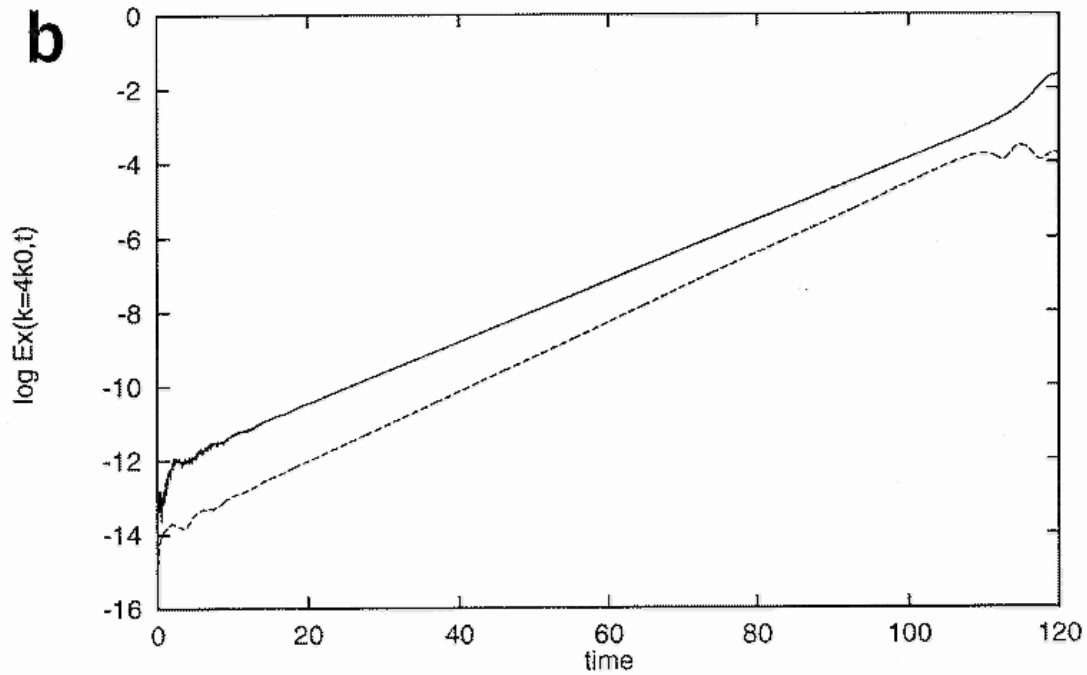
Figure 2: Time evolution of the most unstable plasma modes ( 3\Delta k in (a) and 4\Delta k in (b)) in the case of the parametric decay of the pump wave in the relativistic regime. A logarithmic scale has been used. Full lines correspond to the TSS whereas dotted lines are related to the semi-lagrangian model with full 2D advection using B-splines interpolations.
