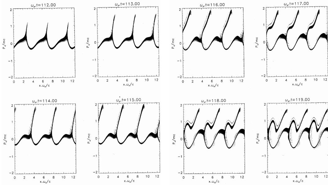
Figure 4: Corresponding x - p_x electron phase space representation of the distribution function computed through 2D full advection and 2D B-spline interpolations. The comparison with Fig. 3 also makes it clear that TSS cannot be adequate here since it leads to numerical instability after time t\omega_p 120 at the saturation of the relativistic modulational instability.
