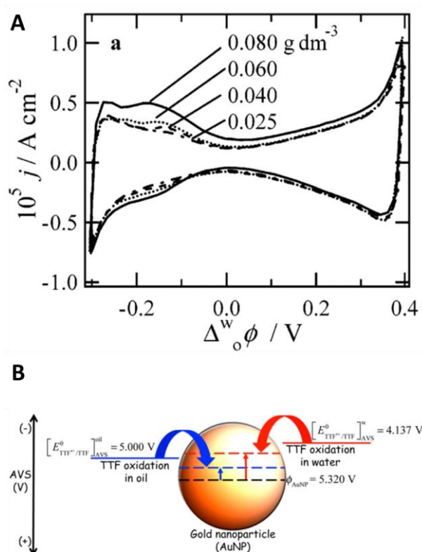
Figure 3. (A) NPs adsorption at the liquid-liquid interface followed by cyclic voltammograms at 100 \text{ mV s}^{-1} showing adsorption / desorption of Au NPs observed between -0.2 and -0.1 V; Adapted from ref. [89] (B) Schematic representation of the work function shift of the Au NPs during charge transfer with tetrathiafulvalene to more reducing potentials. AVS stands for absolute vacuum scale, which corresponds to the scale for the absolute energy positions of the conduction and valence bands, Adapted from ref. [91]
