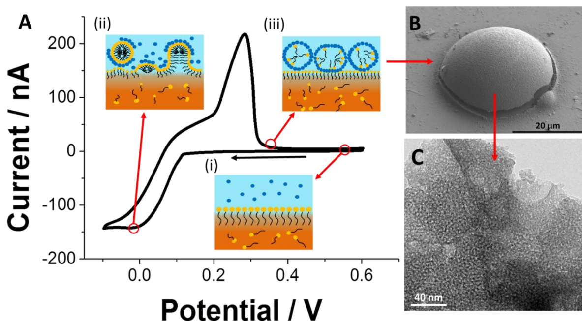
Figure 5. (A) Cyclic voltammogram recorded during silica electrogeneration at the ITIES. Aqueous phase was 50 mM hydrolyzed TEOS and 5 mM NaCl at pH ~ 9.5; Organic phase was 10 mM BTTPPA + TPBCl - and 14 mM CTA + TPBCl - ; Scan rate was 5 mV/s. Silica formation steps: (i) Beginning of polarization, no ion transfer reaction; (ii) CTA + org→aq followed by self-assembly with the hydrolyzed TEOS species; (iii) interfacial deposition and adsorption of CTA +
