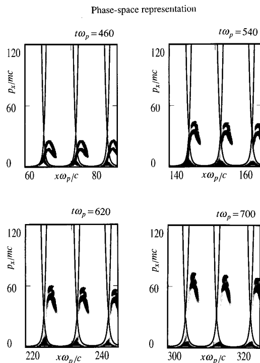
FIG. 14. Representation at different times, of the first window (1) of Fig. 12, moving at the phase velocity of the plasma wave, together with the separatrix of particle orbits. This window has been chosen initially in a region of the modest electric field at the beginning of the instability (the instability has not still reached its strongly nonlinear regime). The particle acceleration behaves in an adiabatic way leading to the acceleration level till p_x/mc \geq 60 .
