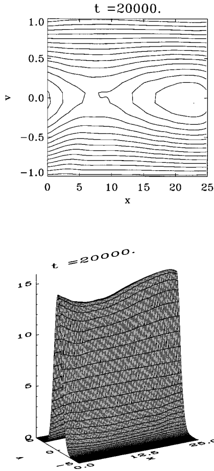
FIG. 15. Distribution function in the phase space (x, V_{||}) for the same case as Fig. 13 at t=20000 .
