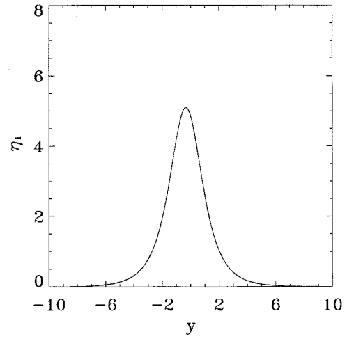
FIG. 2. Typical profile of \eta_i(y) = d \log T_i / d \log n_i .
