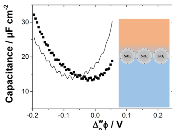
Figure 2: Potential dependence of the interfacial capacitance for the blank cell (solid line) and for (■) 0.5 \text{ g L}^{-1} of silica nanoparticles with a denser aqueous phase. Electrochemical cell 4.
