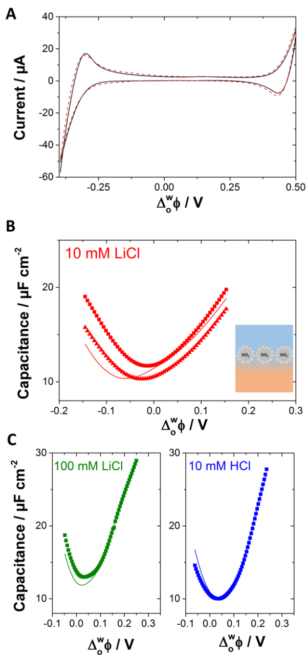
Figure 1: (A) Cyclic voltammetry in the absence (black solid line) and in the presence (red dashed line) of 0.5 g L -1 of silica nanoparticles in the aqueous phase. Electrochemical cell 1, v = 5 \text{ mV s}^{-1} ; (B) Potential dependence of the interfacial capacitance for the blank cell (red solid line) and for (▲) 0.05 and (■) 0.1 g L -1 of silica nanoparticles. Electrochemical cell 1. (C) Potential dependence of the interfacial capacitance for the blank cell (solid line) and for (■) 0.1 g L -1 of silica nanoparticles with 100 mM LiCl (Electrochemical cell 2) or 10 mM HCl (Electrochemical cell 3) as an aqueous electrolyte solution.
