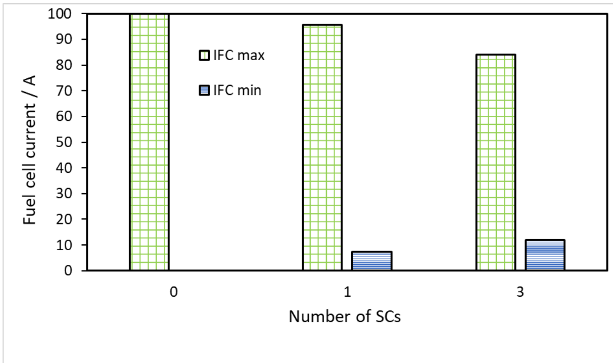
Fig. 3 Effect of SC number on I_{FC}^{\max} and I_{FC}^{\min}
