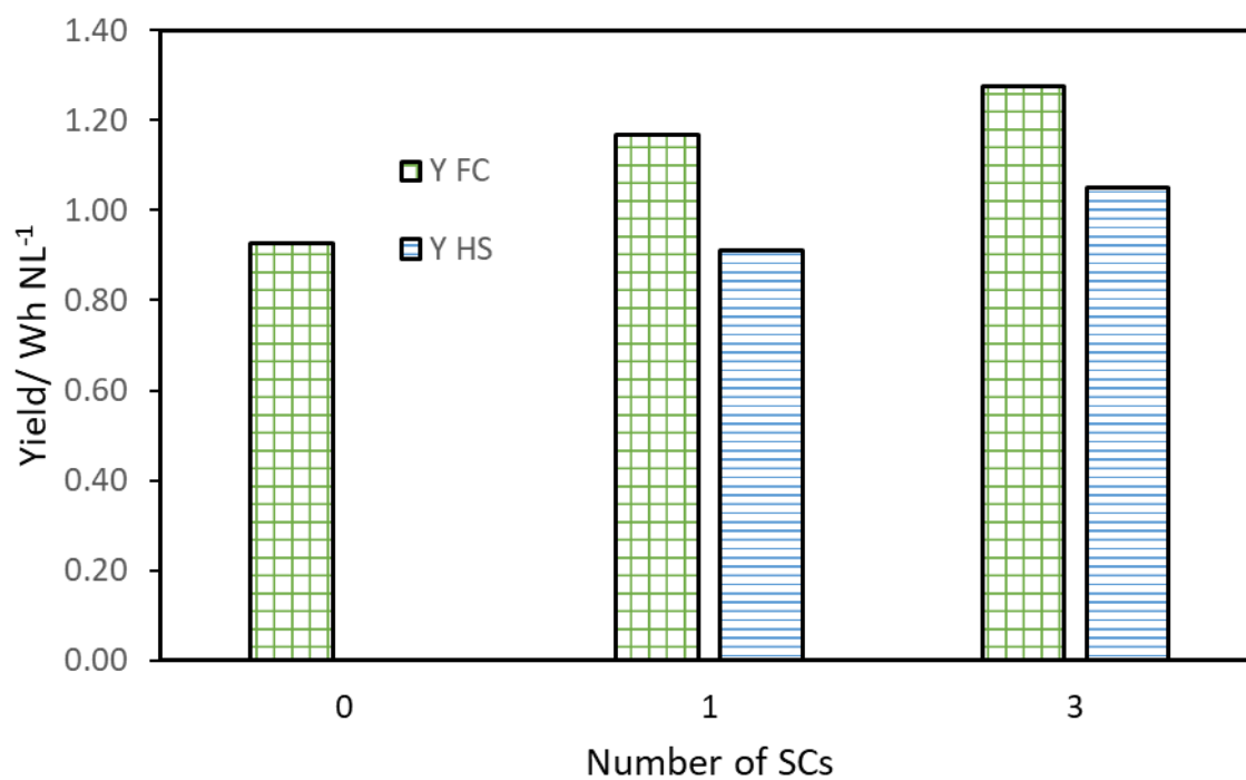
Fig. 8 Effect of the SC number on the yields of the cell and of the hybrid source.
