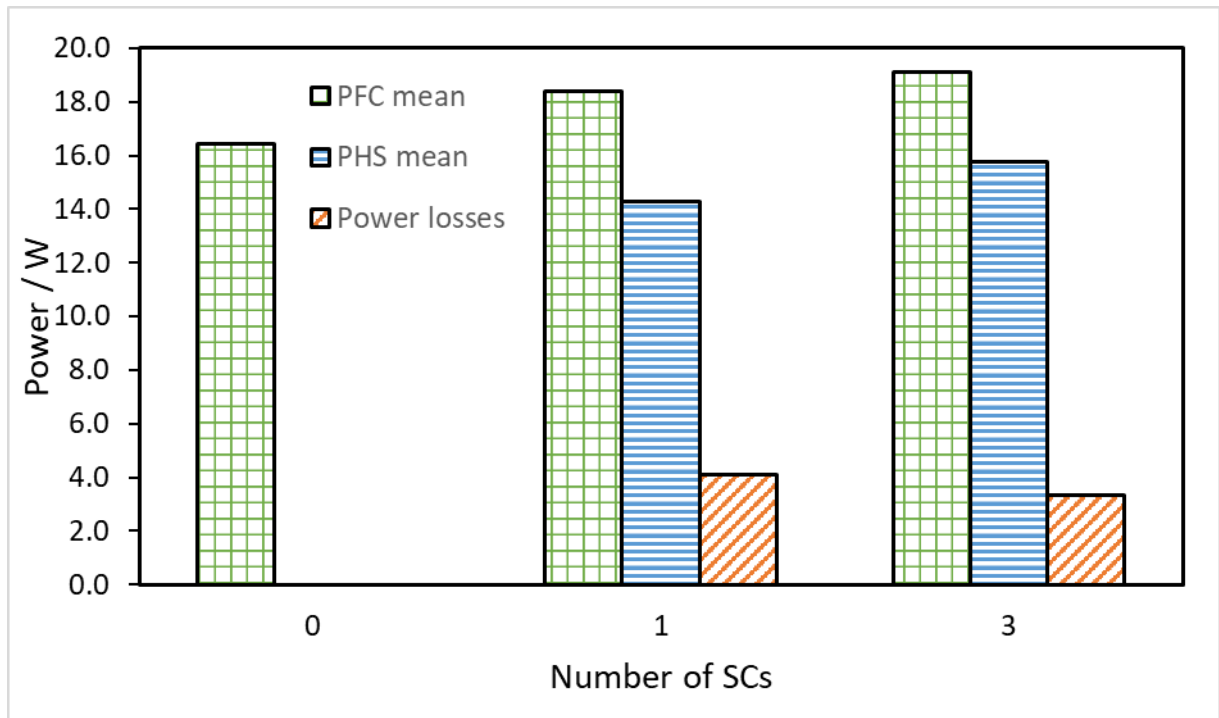
Fig. 5 Effect of the SC number on the mean power and power losses.
