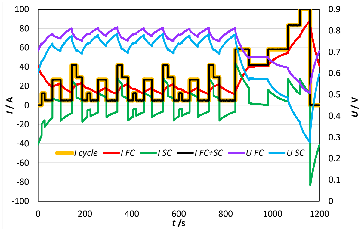
Fig. 4 Current delivered by the 100 cm 2 cell ( I_{FC} ), current passing through the supercapacitor ( I_{SC} ), with the cycle current, together with the cell and SC voltages for a FC-DLC cycle with hybridization (at 200 h).
