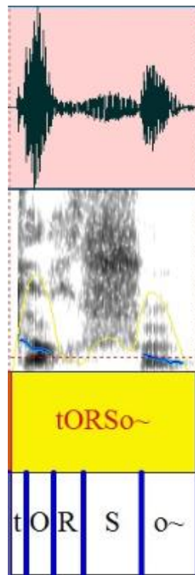
Figure 25 : Spectrogramme de [tORSo~]
