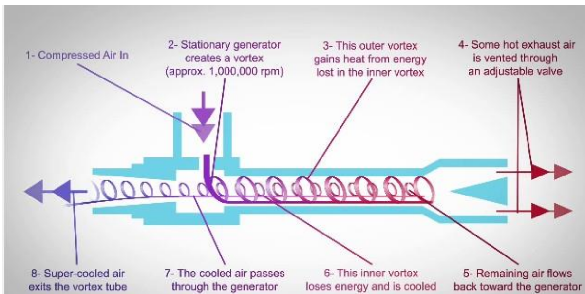
Figure 3 - Tube Ranque
