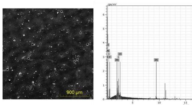
Figure 18. SEM-EDX analysis of the MEA's electrode used as counter electrode after deposition experiment in BMIM TFSI + BMIM Cl 0.1 M at 100 °C, E applied = - 0.7 V vs Ag + /Ag. SEM and EDX analysis of Figure 17 highlight that platinum has been electrodeposited on the working electrode. Figure 18 shows that traces of platinum still remain on the MEA's electrode, but the leaching is almost complete. The platinum can be electrodeposited during MEA's electrode leaching by using a Pt containing leaching solution and controlling the cathode potential.
