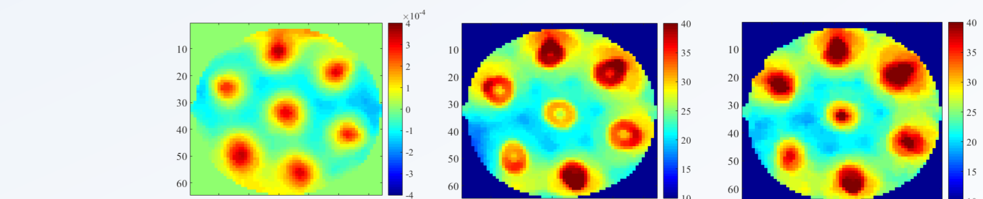
Comparison between velocity (left) and temperature images obtained without outside saturation (center) and with this procedure (right). The images were obtained for \Delta T=36^\circ\text{C} in xanthan.
