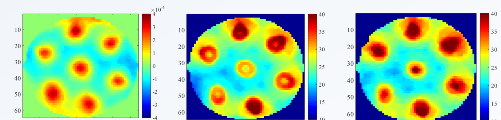
Comparison between velocity (left) and temperature images obtained without outside saturation (center) and with this procedure (right). The images were obtained for \Delta T=36^\circ\text{C} in xanthan.
