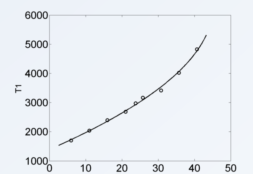
Calibration curves for T1 in a 0,15% xanthan solution as a function of temperature
