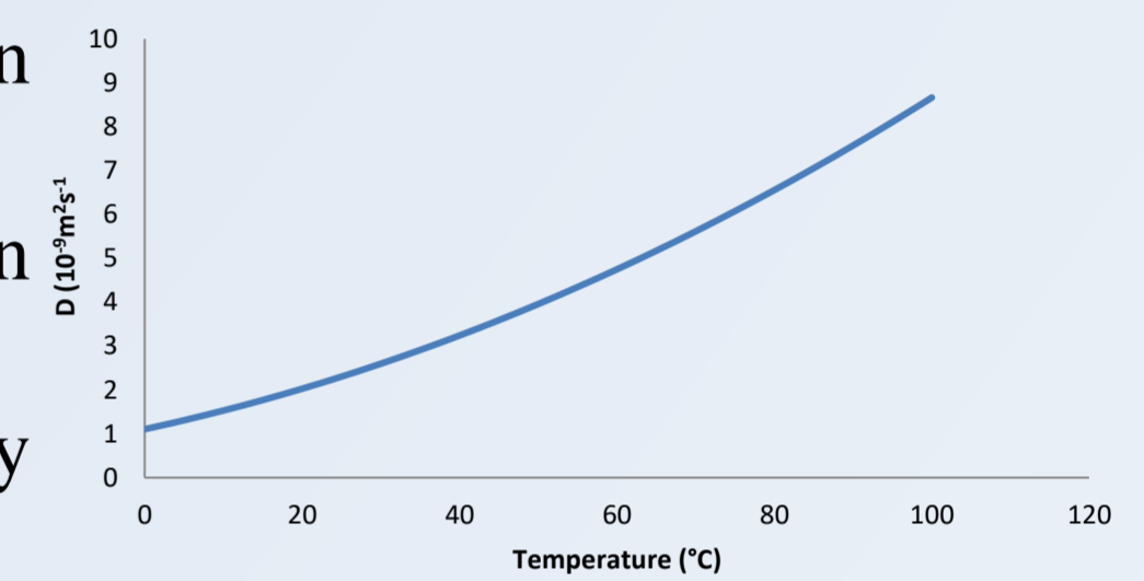
Self diffusion coefficients of water as a function of the temperature
