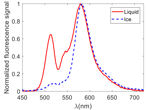
Fig. 8 LIF spectra of Kr/Rh560 dissolved in liquid and frozen water.
