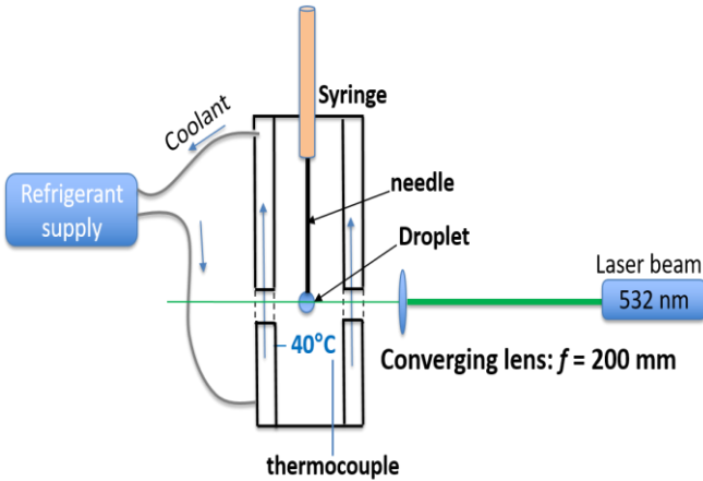
Fig. 5 Calibration setup on a suspended droplet
