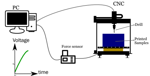
Figure 7: Schematic representation of the drilling experimental set-up.
