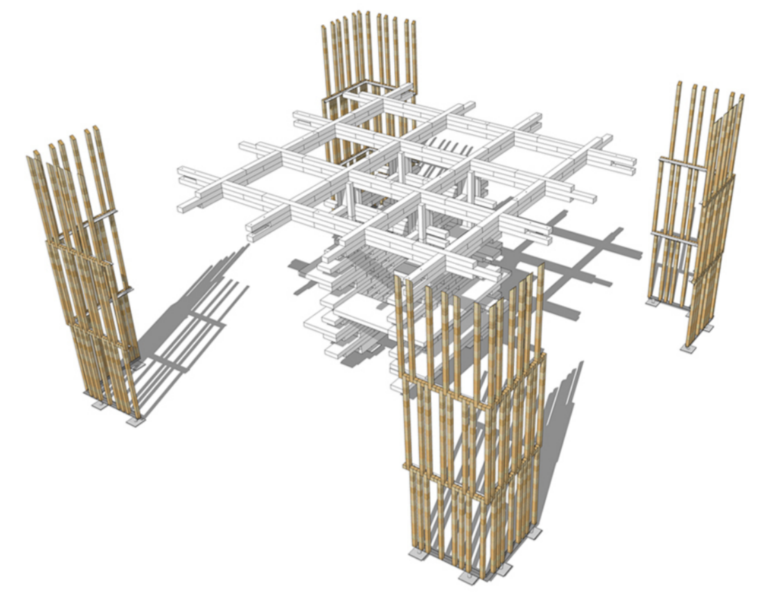
INSTALLATION DES POTEAUX
