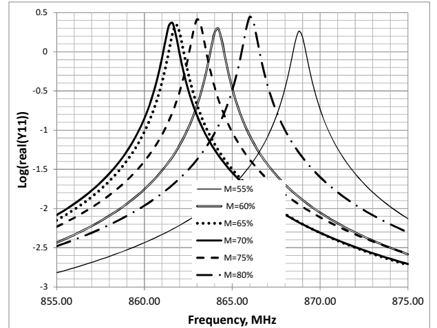
Fig. 7. Details of the modeled dependence of an infinite IDT admittance on metallization ratio; the structure is made with Ir electrode thickness equal to 10% of the IDT period on AlN substrate.
