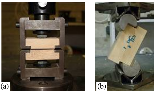
Figure 6 mechanical tests of joints obtained by RSD, (a) shows a test of tensile strength, and (b) shows a test of shear strength
