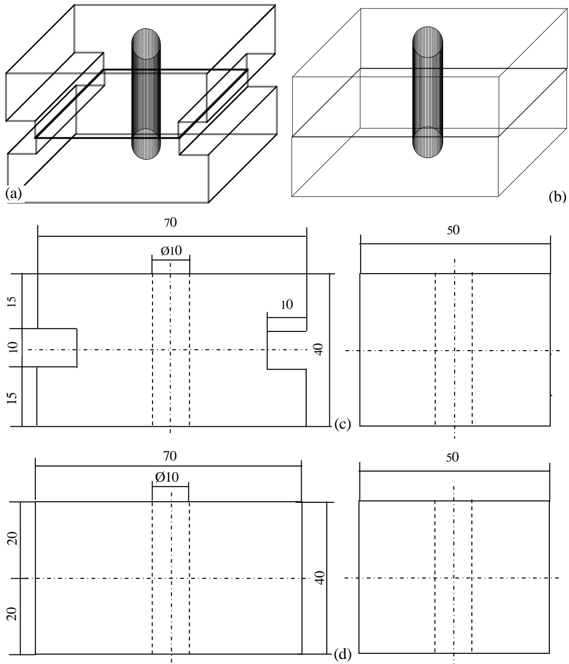
Figure 3 assemblage and size of samples for RDW (a) is a joint for testing the tensile strength, (b) is a joint for the shear strength, (c) presents the dimension of the tensile strength, and (d) presents the dimension of the shear strength samples were conditioned for one week in an environmental chamber (20°C and 65% RH) before testing. The parameters which were varied in the various experiments were: the welding time, maintained after the welding vibration had stopped, the welding pressure exerted on the surfaces, the holding pressure exerted on the surfaces after the welding vibration had stopped, and the amplitude of the shift imparted to one surface relative to the other during vibrational welding. The different welding parameters studied are shown in table 3. For every variation, at least five tests were carried out. For LVW, other specimens(70×50×20mm) are made by a finger-joint. The surfaces to be joined were grooved prior to welding with a milling cutter. Different types of grooves
