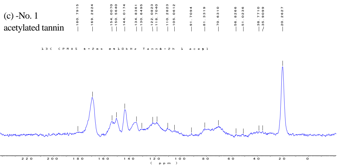
Figure 13 CPMAS ^{13}\text{C} NMR solid state spectra of (a) No. 3 acetylated tannin, (b) No. 2 acetylated tannin, (c) No. 1 acetylated tannin
