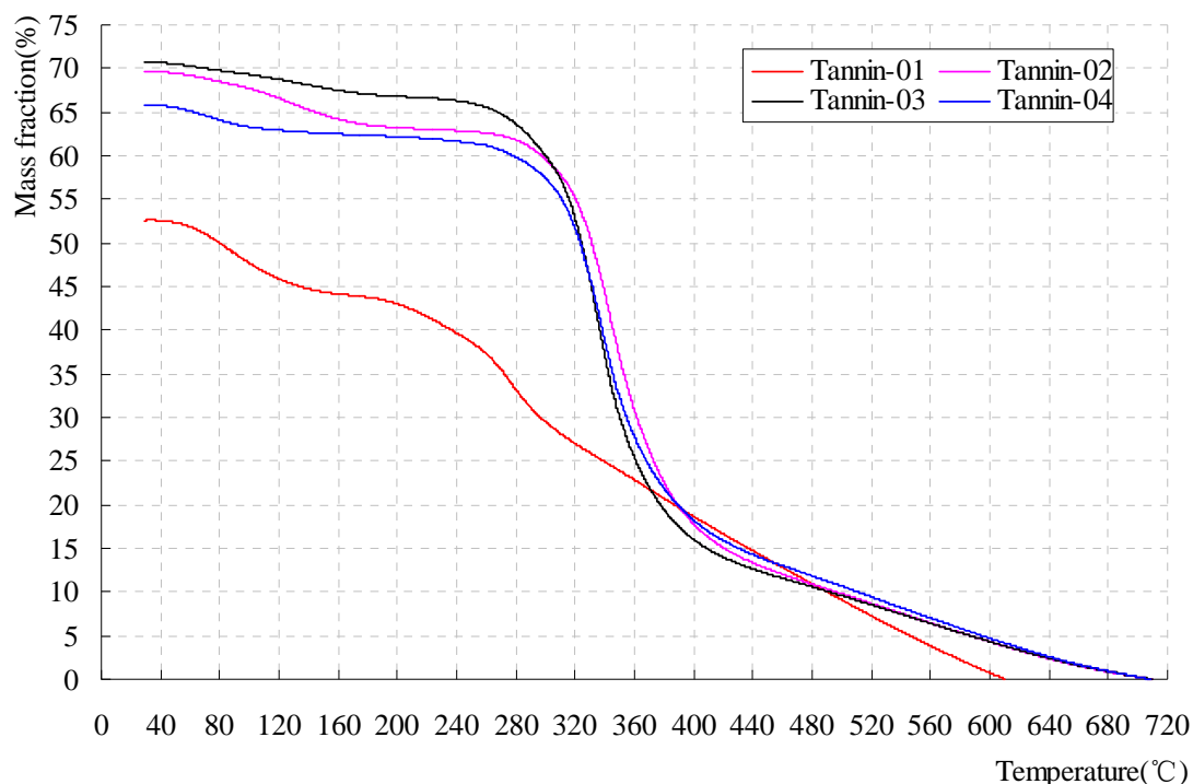
Figure 16 TG curves of tannin and three acetylated tannin in nitrogen (N 2 ) atmospheres
