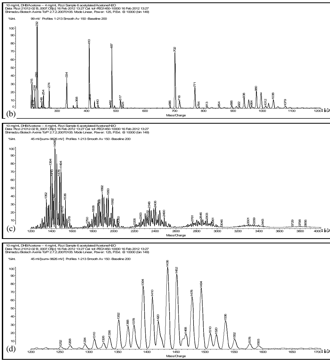
Figure 15 (a) MALDI-TOF of tannin 8h-acetylated with pyridine in the 75-210 Da range, (b) MALDI-TOF of tannin 8h-acetylated with pyridine in the 210-1200 Da range, (c) MALDI-TOF of tannin 8h-acetylated with pyridine in the 1200-4000 Da range and (d) MALDI-TOF of tannin 8h-acetylated with pyridine in the 1200-1700 Da range
