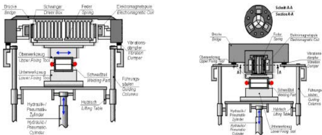
Figure 2 description and diagrams of vibration welding technologies (Gerber et al. 2000)
