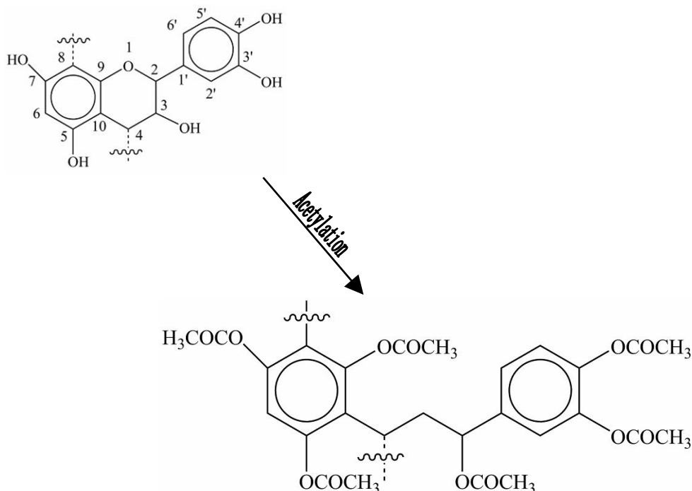
Figure 12 acetylation of tannin
