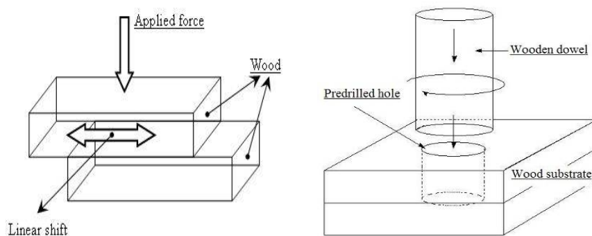
Figure 1 Schematic representation of the vibrational movements of two solid wood surfaces (Left), Schematic representation of the insertion of a cylindrical dowel in a predrilled hole of wood substrate (Right) (Gfeller et al. 2004, Pizzi et al. 2004)
