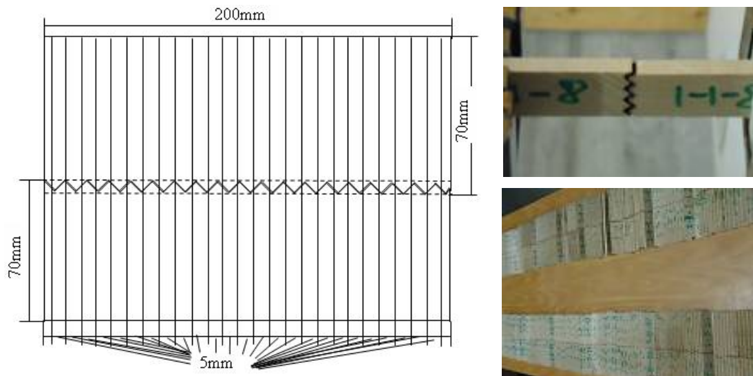
Figure 7 sawing the jointed pieces of grooved surface for the mechanical tests
