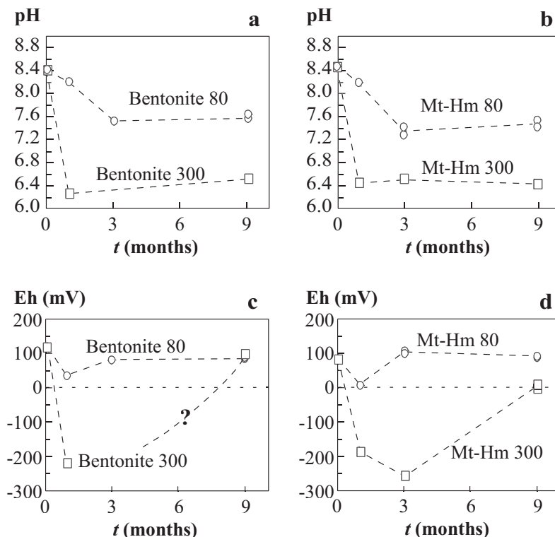
FIG. 9. Chemistry of the run solutions: (a–b) evolution of pH vs. time for ‘Bentonite’- and ‘Mt-Hm’-type experiments, respectively. (c–d) Evolution of Eh vs. time for ‘Bentonite’- and ‘Mt-Hm’-type experiments, respectively.
