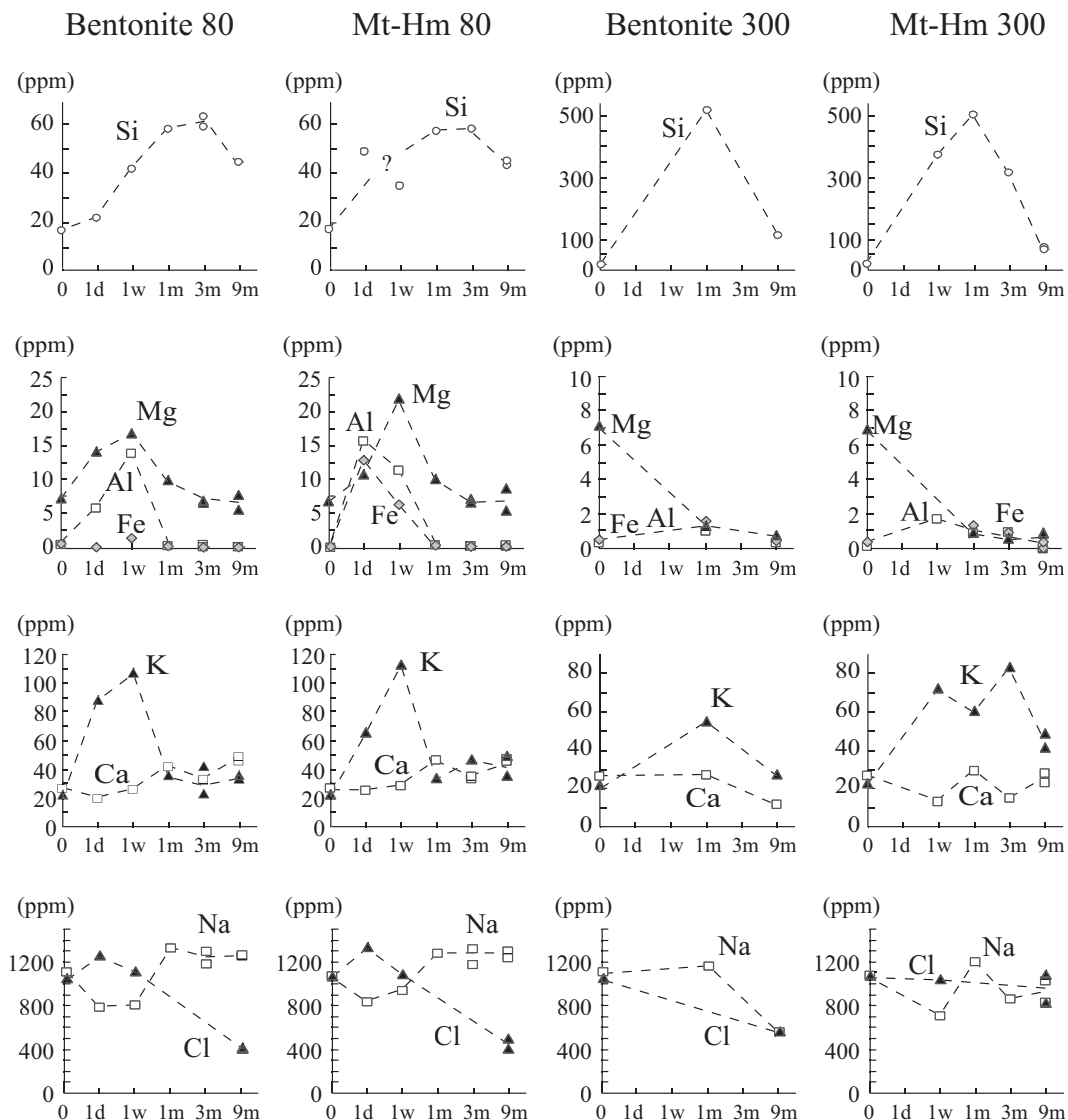
FIG. 10. Chemistry of the run solutions. Evolution with time of the solution composition (ppm scale) for different cations (Si, Al, Fe, Mg, K, Ca, Na and Cl) and the four different experimental conditions. 1d = 1 day, 1w = 1 week, 1m = 1 month, 3m = 3 months, 9m = 9 months.
