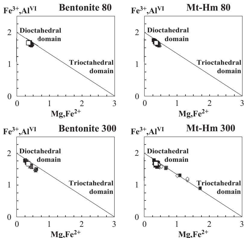
FIG. 8. Chemistry of the clay phase of the starting sample (open square), 1 month (filled triangles), 3 months (open diamonds) and 9 months (filled squares) run samples. ( \text{Fe}^{3+}, \text{Al}^{\text{VI}} ) vs. ( \text{Fe}^{2+}, \text{Mg} ), from structural formulae calculated on the basis of 11 Oxygens.
