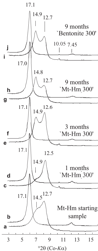
FIG. 3. XRD patterns of the Mt-Hm starting-sample, 1 month, 3 months and 9 months 'Mt-Hm 300' run samples, and 9 months 'Bentonite 300' run sample. (a, c, e, g, i) oriented air-dried; (b, d, f, h, j) EG-saturated. Reflection values in \text{\AA} .
