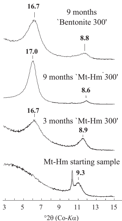
FIG. 4. XRD patterns of the Mt-Hm starting sample, 3 months and 9 months 'Mt-Hm 300' run samples, and 9 months 'Bentonite 300' run sample, after Greene-Kelly test. Reflection values in Å.
