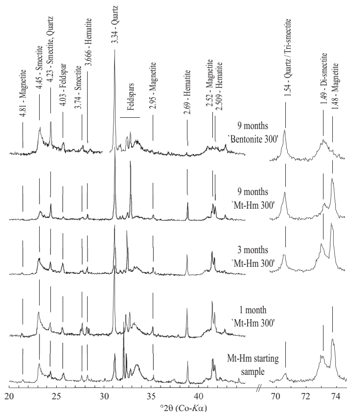
FIG. 1. XRD powder patterns of the Mt-Hm starting sample, 1 month, 3 months and 9 months 'Mt-Hm 300' run samples, and 9 months 'Bentonite 300' run sample. Reflection values in Å.
