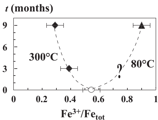
FIG. 5. Evolution of the \text{Fe}^{3+}/\text{Fe}_{\text{tot}} ratio in the clay phase of the run samples measured by TMS vs. experimental duration. Dark diamonds: 'Mt-Hm 300' experiments; dark triangle: 'Mt-Hm 80' experiment; open circle: comparison with the \text{Fe}^{3+}/\text{Fe}_{\text{tot}} ratio in the starting montmorillonite (Guillaume et al. , 2001b).
