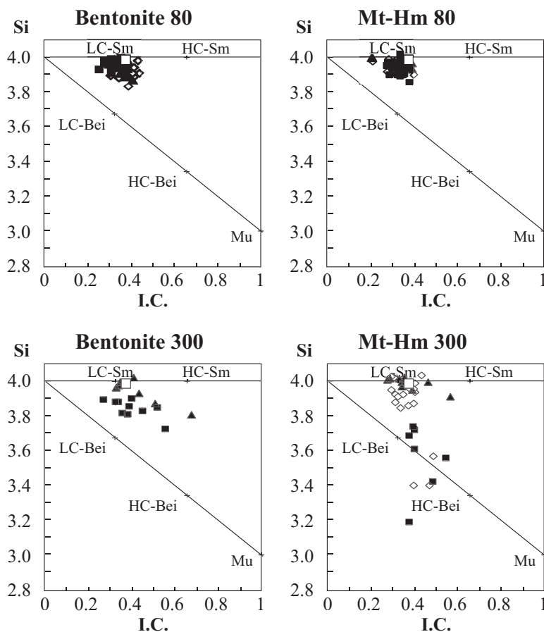
FIG. 6. Chemistry of the clay phase of the starting sample (open square), 1 month (filled triangles), 3 months (open diamonds) and 9 months (filled squares) run samples. Si vs. interlayer cations (I.C. = \text{Na}+2\text{Ca}+\text{K} ), from structural formulae calculated on the basis of 11 oxygens. Reference minerals are reported: low-charge and high-charge smectite (LC-Sm, HC-Sm), low-charge and high-charge beidellite (LC-Bei, HC-Bei), Muscovite (Mu).
