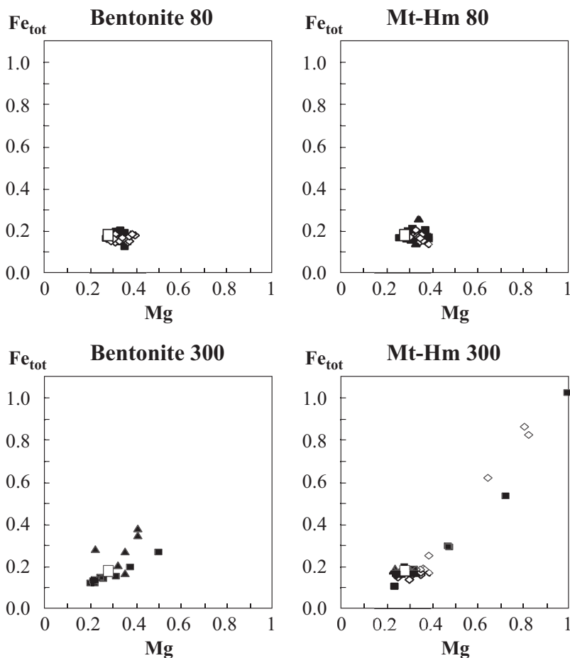
FIG. 7. Chemistry of the clay phase of the starting sample (open square), 1 month (filled triangles), 3 months (open diamonds) and 9 months (filled squares) run samples. Fe total vs. Mg, from structural formulae calculated on the basis of 11 oxygens.
