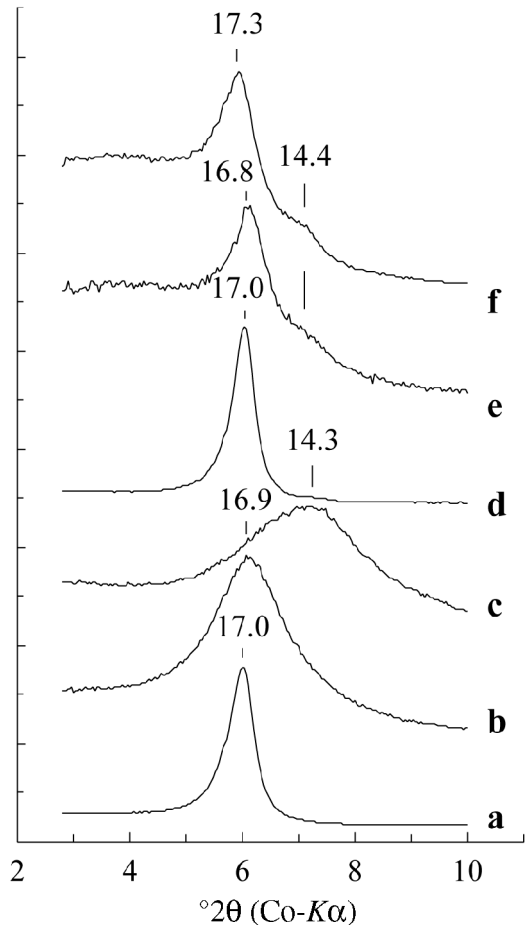
Fig. 6. XRD patterns of Li-, K- and Mg-saturated samples. (a, b) starting sample, (a) Li- then EG-saturated, (b) K-saturated, 110°C heated then EG-saturated; (c, d) 9 months WIP run sample, (c) K-saturated, 110°C heated then EG-saturated, (d) Mg- then glycerol-saturated; (e, f) 9 month IP run sample, (e) Li- then EG-saturated, (f) Mg- then glycerol-saturated. Reflection values in Å.
