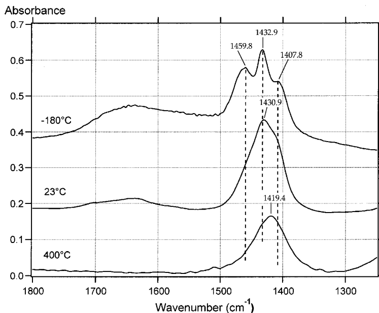
FIG. 4. FTIR spectra of the NH_4^+ -bending vibrations of tobelite recorded with the IR microscope at different temperatures.
