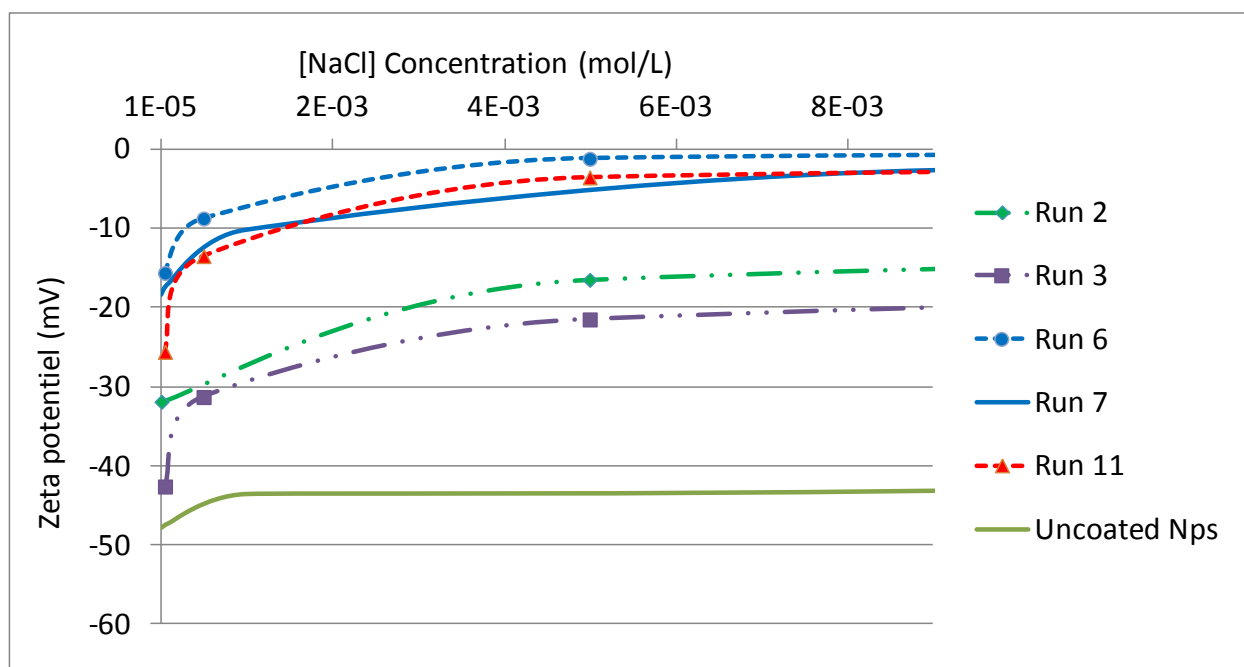
Figure 2. Evolution of zeta potential for NPs made by nanoprecipitation of Dex-g-PNBA (Runs 2 and 3, Table 1) or by emulsion/evaporation with (or not) in situ CuAAC (Runs 6, 7 and 11, Table 1) against concentration of NaCl.
