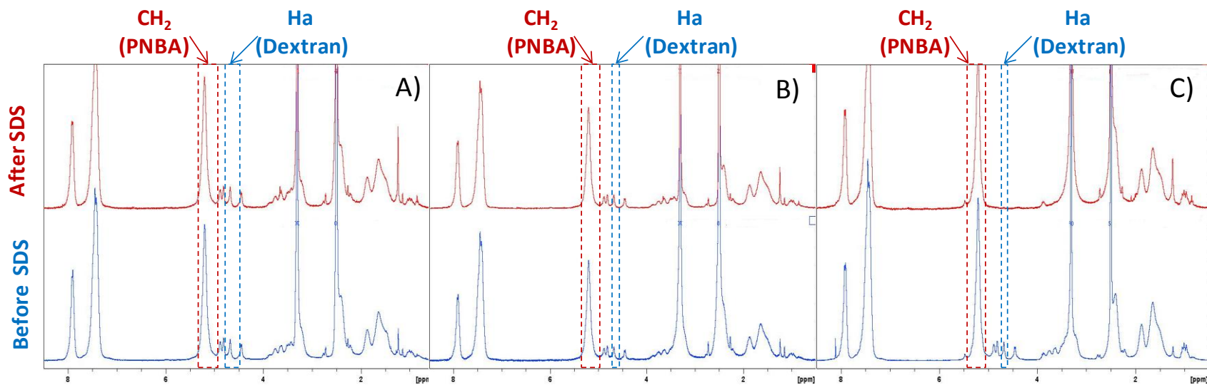
Figure 3. ^1\text{H} NMR spectra ( \text{DMSO-}d_6 ) of NPs produced with (A, B) or without (C) in situ CuAAC. Click chemistry was carried out under (A) or without (B) \text{N}_2 flow. Spectra are given before and after SDS contact.
