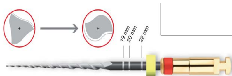
Figure 25 : One Shape® New Generation (MICRO-MEGA®, 2015).
