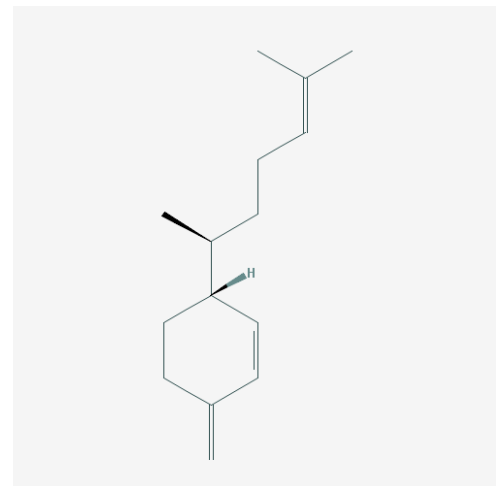
Figure 57 : \beta -sesquiphellandrene (PubChem, https://pubchem.ncbi.nlm.nih.gov , 2016)
