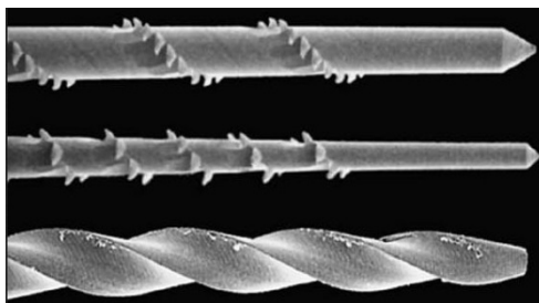
Figure 9 : Profil des instruments Sonic Air® (source : http://pocketdentistry.com/wp-content/uploads/285/9783131469922_c012_f001.jpg )
