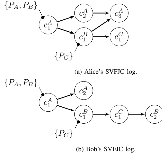
Figure 5. Bob ( P_B ) invites Carol ( P_C ) in his contribution c_1^B . Carol issues c_1^C which depends on c_1^B . In the meantime Alice ( P_A ) issues c_2^A which is concurrent with Bob's and Carol's contributions. Alice receives c_1^B and c_1^C , when Bob receives the contribution of Carol before the contribution of Alice. (a) and (b) respectively depicts the SVFJC log of Alice and Bob.
