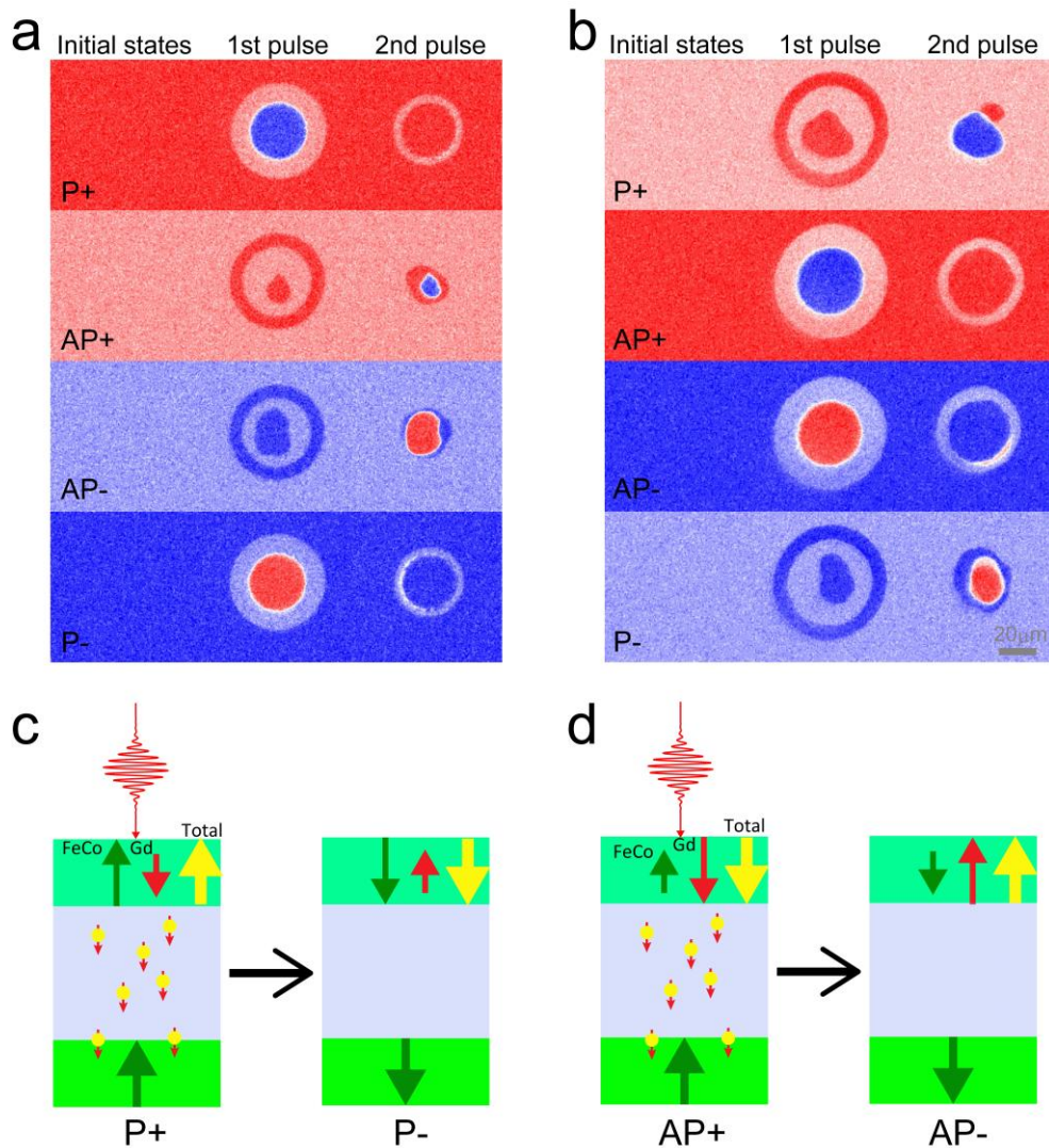
Figure 4. (All-Optical Switching in GdFeCo / Cu / [Co/Pt] spin-valves with different GdFeCo concentration. a) AOS results for FeCo-rich Gd 23.3 (FeCo) 76.7 (5 nm) / Cu(9.3 nm) / [Co/Pt] 4 sample. b) AOS results for Gd-rich Gd 26.4 (FeCo) 73.6 (5 nm) / Cu(10 nm) / [Co/Pt] 4 sample. Since MOKE is more sensitive to the FeCo magnetic sublattice, the magnetic contrast signals of AP+ states are larger than that of P+ state in the case of spin-valve sample with Gd-rich GdFeCo. Schematic illustration of spin-polarized hot electron transport induced magnetization switching for c), FeCo-rich and d), Gd-rich GdFeCo / Cu / [Co/Pt] spin valve structures.)
