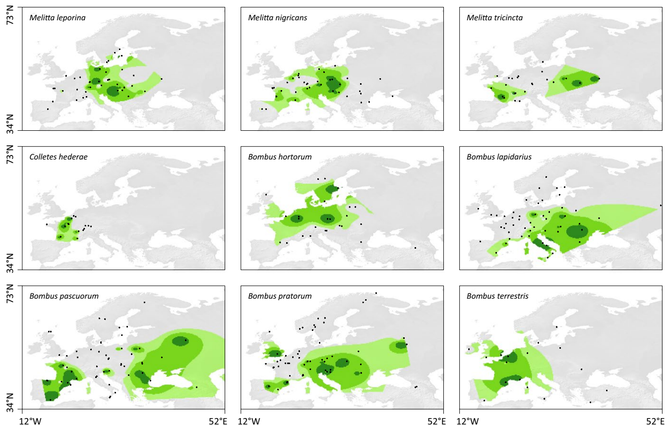
FIGURE 1 For each considered species, areas with nucleotide diversity higher than specific threshold values (0.50, 0.75 and 0.95 quantile values, in shades of increasing darkness). See Material and methods section for a complete description of the method used to generate these surfaces. The black dots are sampled populations with more than two specimens. This figure is based on initial interpolation surfaces based on a sliding window with a radius r = 50 km (see Supporting information Figures S1 and S2 for equivalent figures based on sliding window radius r = 25 and 100 km, and Supporting information Figure S3 for maps displaying variation of genetic diversity among loci) [Colour figure can be viewed at wileyonlinelibrary.com ]
