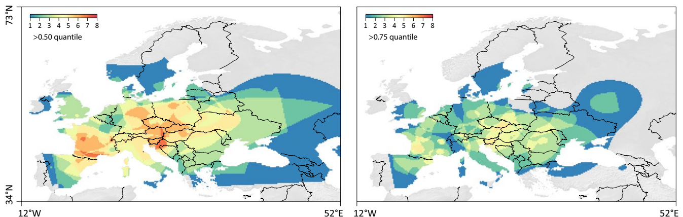
FIGURE 2 Consensus maps based on the specific threshold maps built from interpolation surfaces based on sliding windows with a radius r = 50 km. The colour scale reports the number of species for which the nucleotide diversity is higher than the threshold value of 0.50 and 0.75 quantiles. Black lines indicate the position of national borders. See Supporting information Figure S4 for consensus maps based on alternative sliding window radius [Colour figure can be viewed at wileyonlinelibrary.com ]
