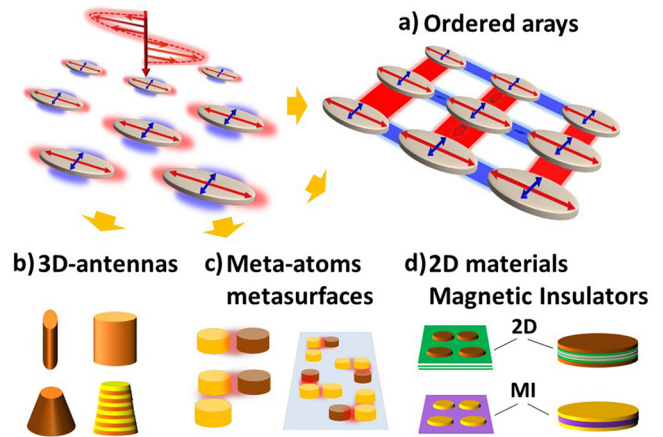
Figure 15. Examples of strategies to increase the MO response of MP materials. (a) Arrangement of MP nanoantennas in ordered arrays to exploit their mutual interaction in the far field [105]; (b) realization of 3D MP nanostructures of different and precisely controlled size and shape [106], made of various materials; (c) design of unit blocks comprising closely-packed multiple materials (high-index dielectrics supporting Mie resonances, NMs and FMs) nanoantennas to profit from their near-field interaction; (d) combination of MP nanostructures with 2D materials and magnetic insulators (MI). Typical size of the MP nanoantennas shown is in the order of 100 nm. (a) Reprinted with permission from [105]. Copyright (2016) American Chemical Society. (b) Reprinted with permission from [106]. Copyright (2014) American Chemical Society.
