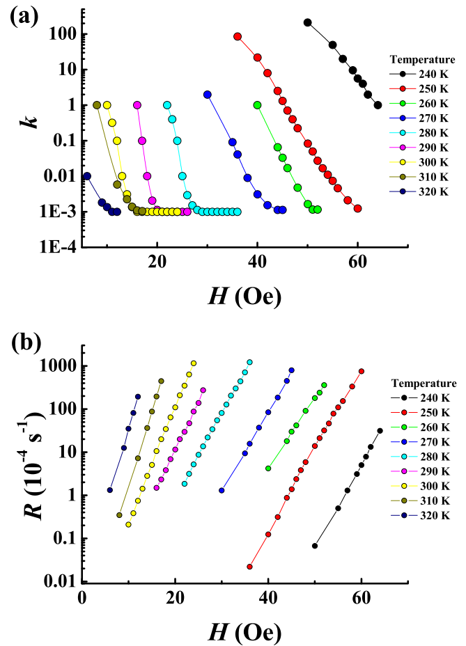
FIG. 5. Magnetic field dependences of propagation constant k (a) and nucleation probability R (b) in the 240–320 K temperature range.
