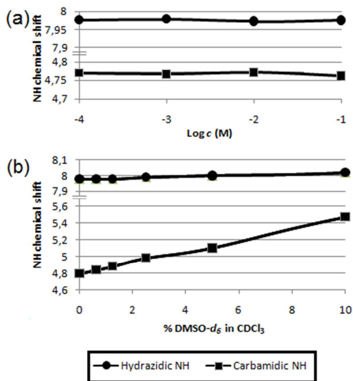
FIGURE 5. (a) Concentration-dependence in CDCl 3 (from 10 -1 to 10 -4 M) and (b) solvent dependence as determined by 1 H NMR (300 MHz) in mixed CDCl 3 /DMSO- d 6 (c = 10 -2 M) of NH chemical shifts of 1
