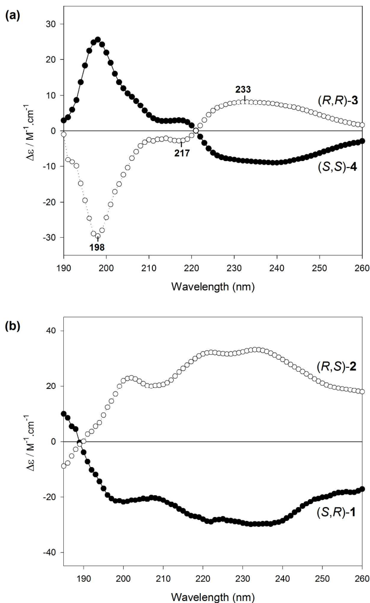
FIGURE 11. Microcrystalline normalized CD spectra of pseudodipeptides 1-4, in Nujol mulls ( c = 25 - 50 \text{ mg} \cdot \text{mL}^{-1} ), in 0.01 cm quartz flat cells, at 293K; Nujol blank was subtracted from the spectra: (a) Superimposition of homochiral compounds (R,R) -3 and (S,S) -4 CD spectra. (b) Superimposition of heterochiral compounds (S,R) -1 and (R,S) -2 CD spectra
