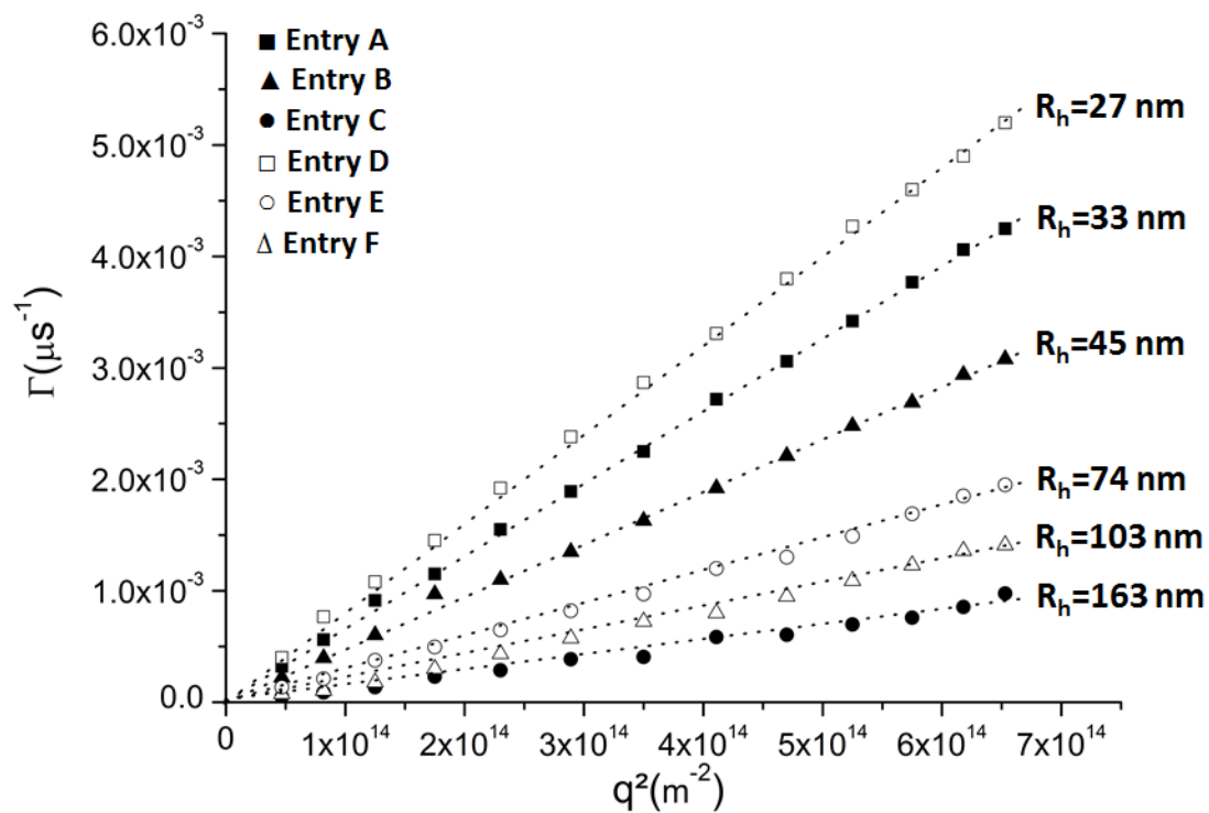
Figure S14. q^2 dependence of the relaxation rate ( \Gamma ) for various Dex- g^5 -PPMA _y nanostructures prepared by photo-PISA of HPMA in aqueous medium using Dex-TTC as the macro-CTA, at different conditions (see Table S1).
